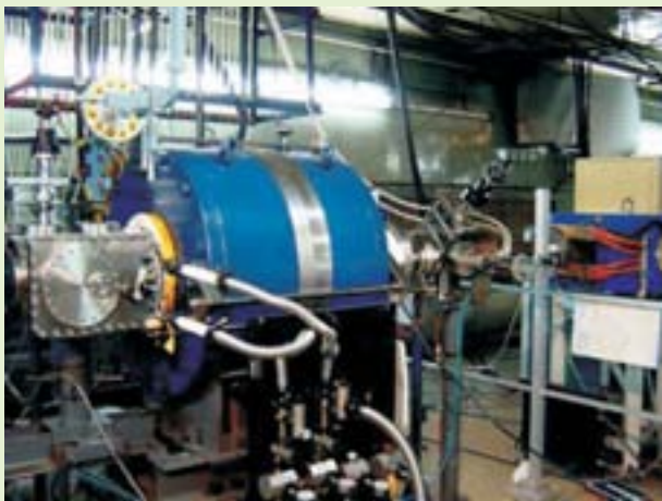
Fig. 2. ECR Ion Source for Radioactive Ion Beam
