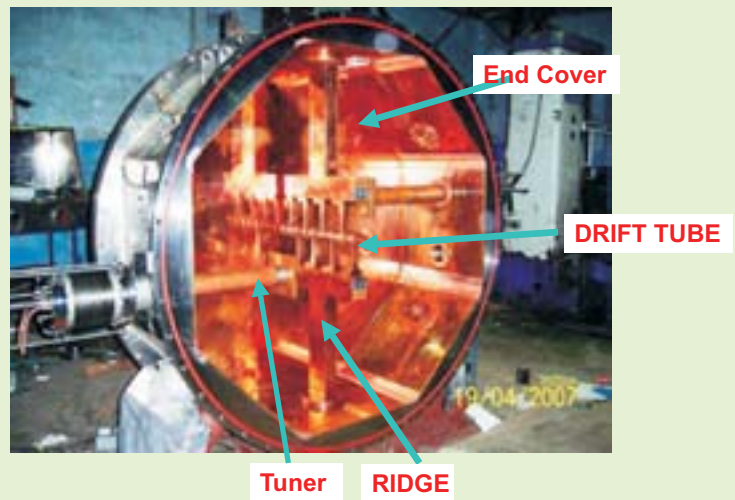
Fig. 5. LINAC during assembly
