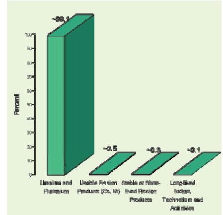
Constituents of spent nuclear fuel
