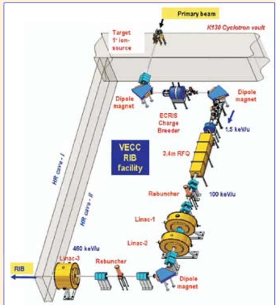
Fig. 1. Schematic layout of RIB facility
