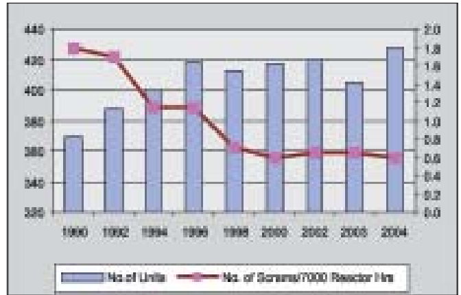
Fig. 6 Unplanned scrams/7000 hrs of Reactor Operation (Based on: Nuclear Power and Sustainable Development, IAEA, April 2006, pg 16)
