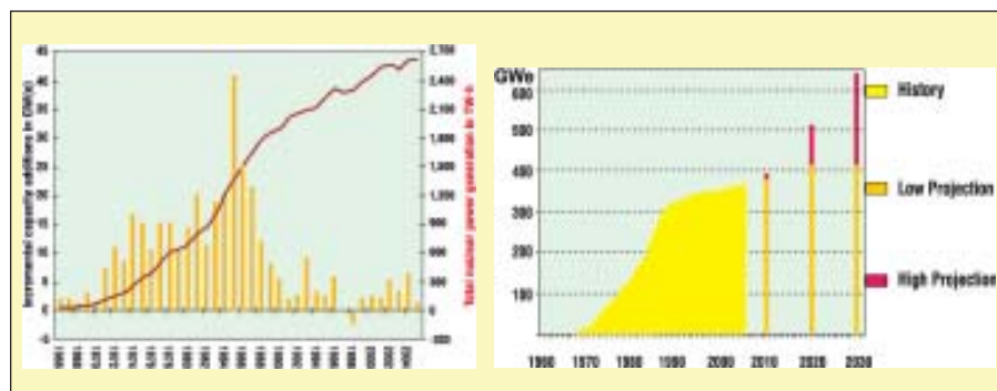
Fig. 3 Nuclear electricity Generation and capacity addition
