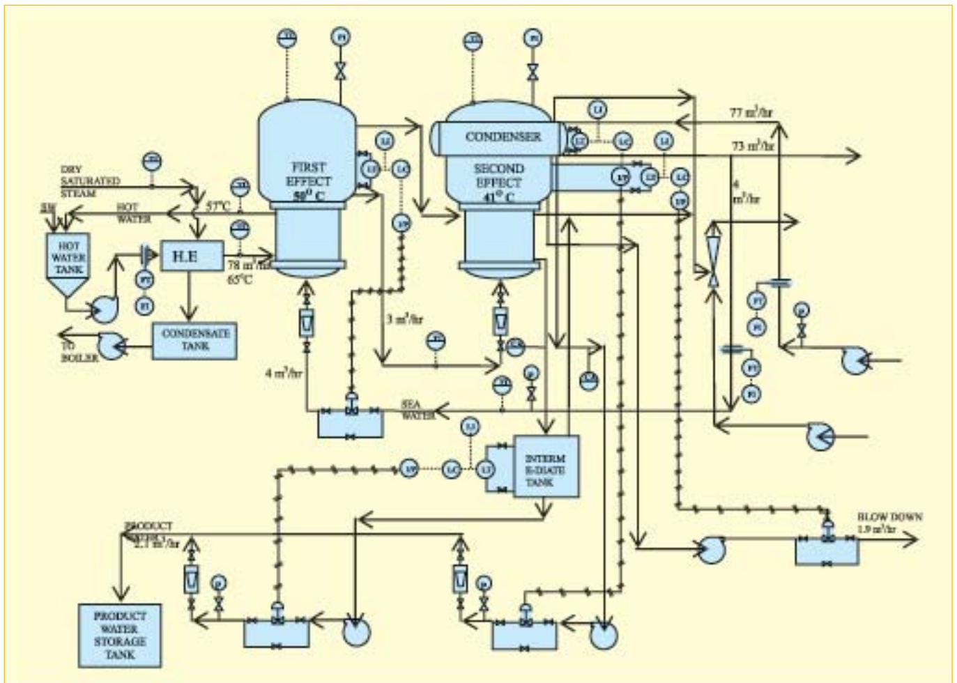
Fig. 1: Process Flow Diagram of 50,000 litres/day 2-Effect LTE Desalination Plant
