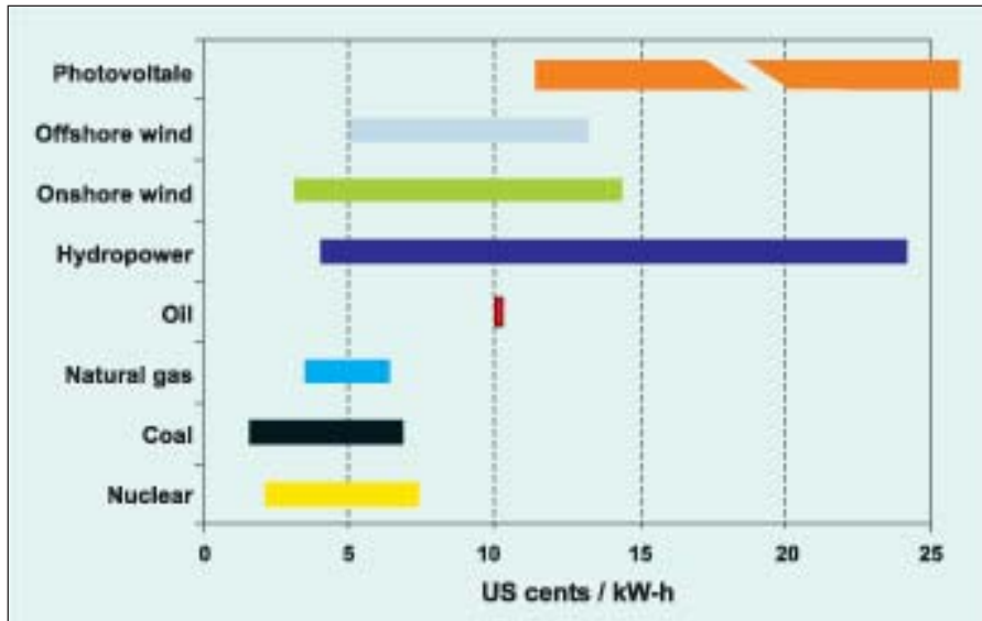
Fig. 8 Levelised electricity cost from new construction (Courtesy: Nuclear Power and Sustainable Development, IAEA, April 2006, pg. 9)
