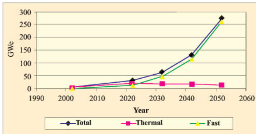
Fig. 8: Nuclear Power Installed Capacity – Type Mix
