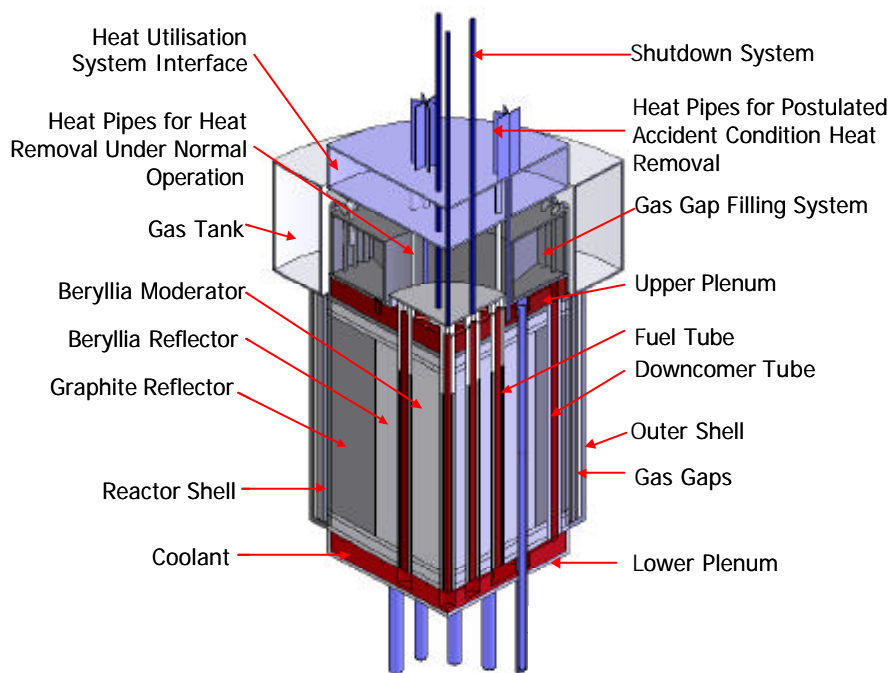
Figure 17: Compact High Temperature Reactor
